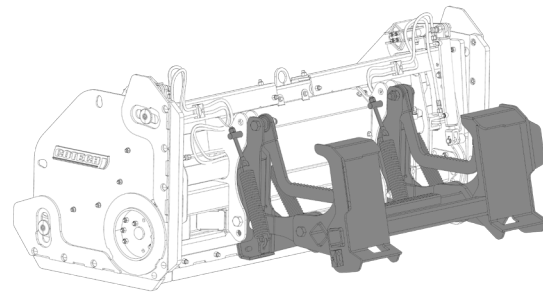
SKST-PP trip system for Skid Steer. Weight 275 lbs.
