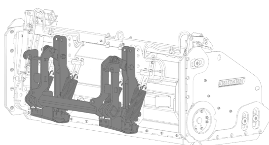
PP-L trip system for loaders. Weight 150-300 lbs depending models
